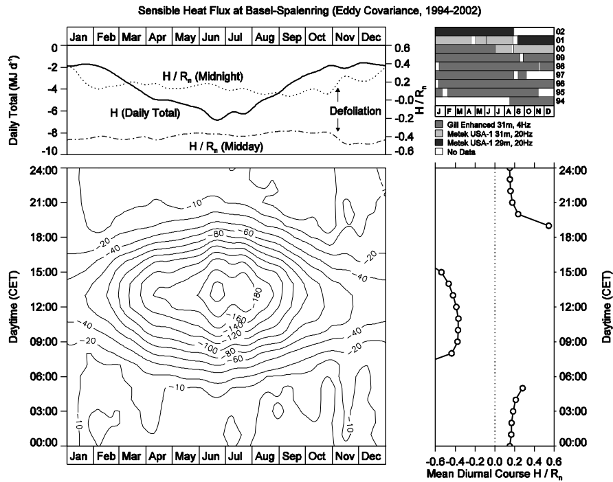
Fig. 4: Results of the long term eddy-covariance measurements. From 1994 to 2002 different eddy-covariance systems measured sensible heat flux at site U2. Main plot: The isofluxdiagram illustrates the climatological averaged values of the sensible heat flux H in dependence of daytime and day of year in W m^2 . The diagram again illustrates that during nighttime all around the year negative heat fluxes are measured (i.e. away from the surface). Right plot: Mean diurnal course of the fraction H/R_n for the period 1994-2002. Upper left plot: Yearly course of the daily total values (full line) and fraction H/R_n for Midday and Midnight. Upper right: Documentation of the different eddy covariance systems that were operated at U2 and contribute to the climatological averaged values.
